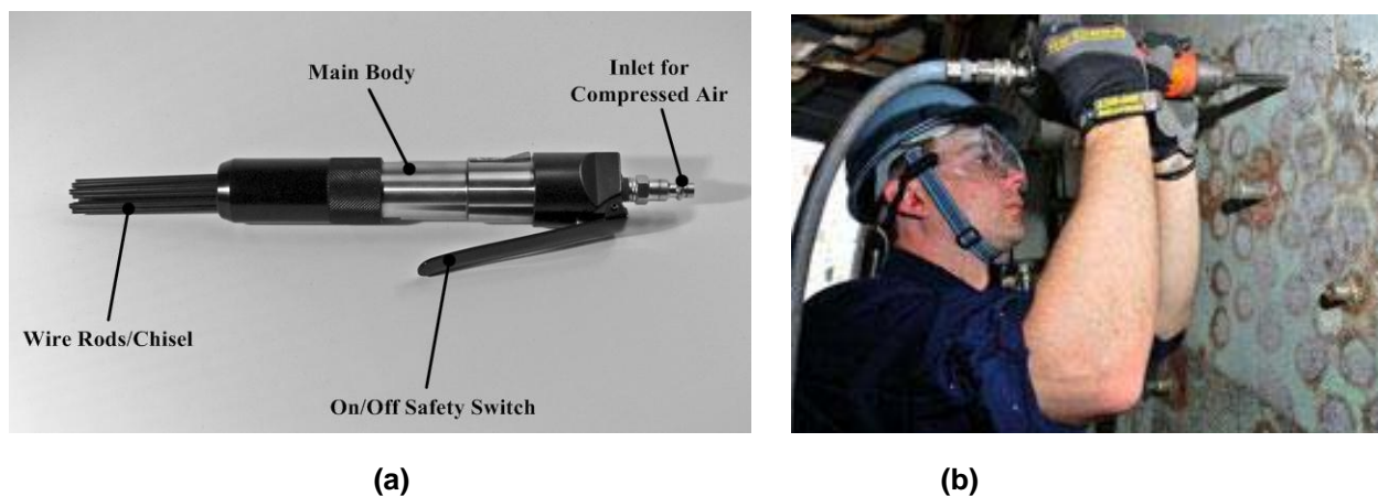
Figure 4 (a) Needle gun used for collecting data reported in Figure 5, and (b) common needle gun cleaning application/environment.
